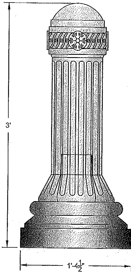
SIDE VIEW SCALE: 1 1/2" = 1'-0" 1
