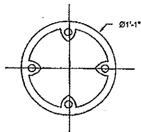
13" 4 HOLE ANCHOR BOLT CIRCLE STANDARD
