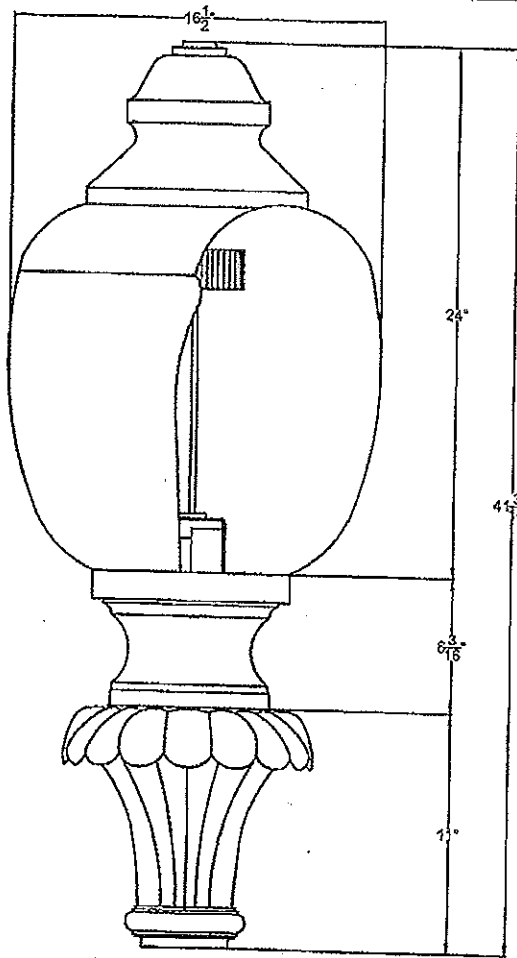
SIDE VIEW SCALE: 1 1/2" = 1'-0" 1
