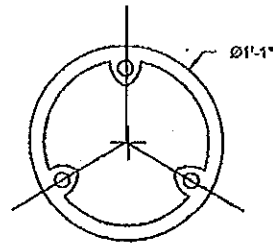
13" 3 HOLE ANCHOR BOLT CIRCLE STANDARD
