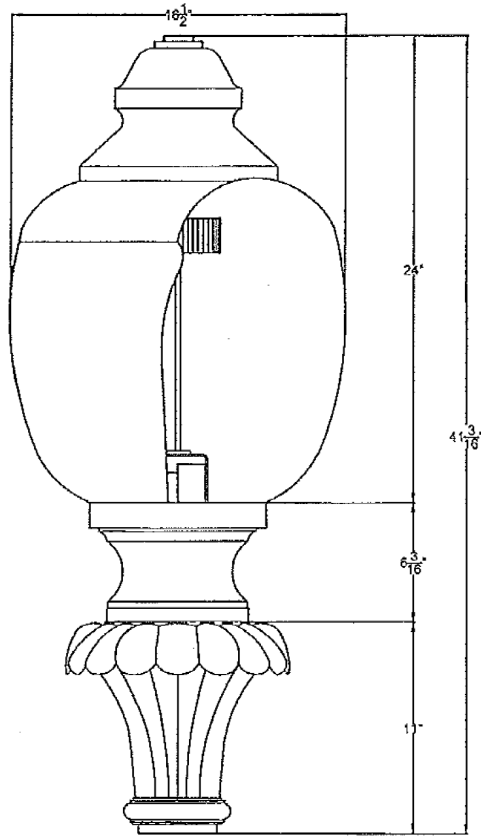
SIDE VIEW 1 SCALE: 1 1/2" = 1'-0"
